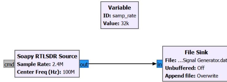
FIGURE 3.7: Blocks used in GNU Radio to save the data from the Yagi Uda Antenna through RTL-SDR
