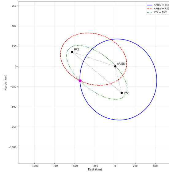
FIGURE 4.12: Target prediction in Bistatic Geometry
