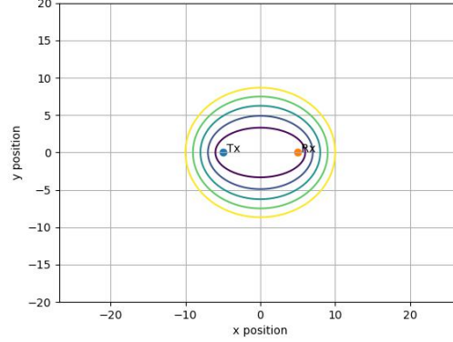
FIGURE 2.2: Family of contours with the transmitter and receivers and focii
