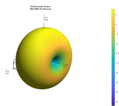
FIGURE 3.16: Phased Array with 2 elements - 3D Plot
